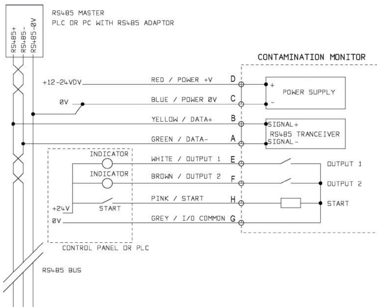
Figure 3: External wiring example
