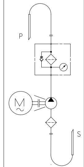
HYDRAULIC CIRCUIT
